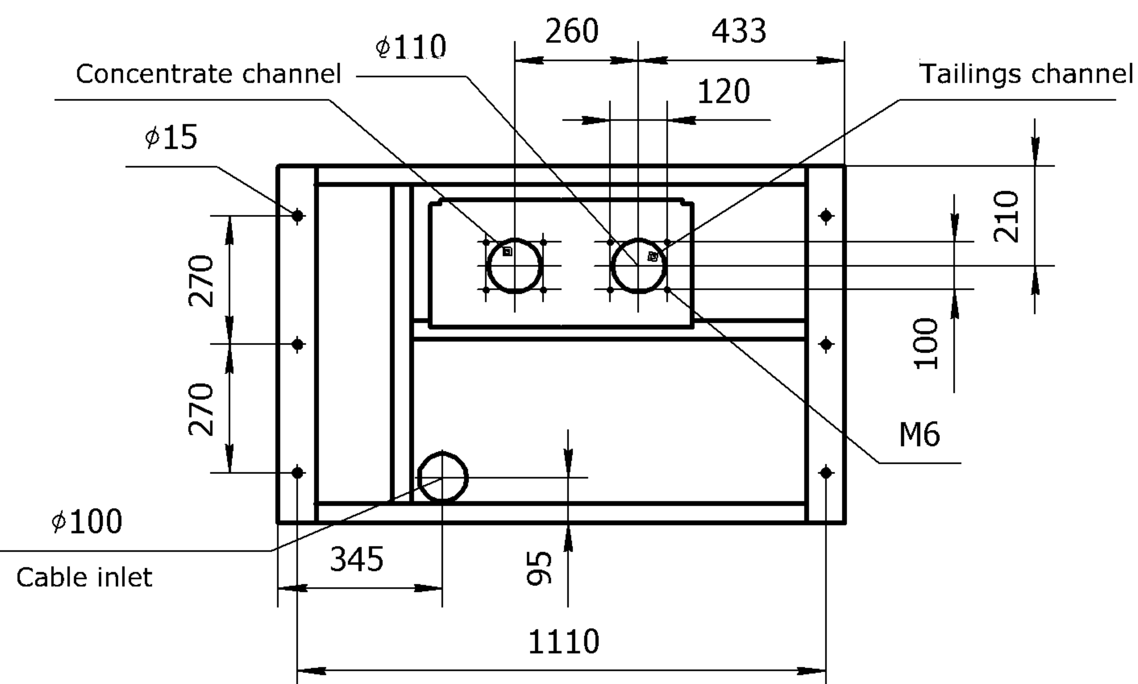
Sorting machine LS-D-4-03P
