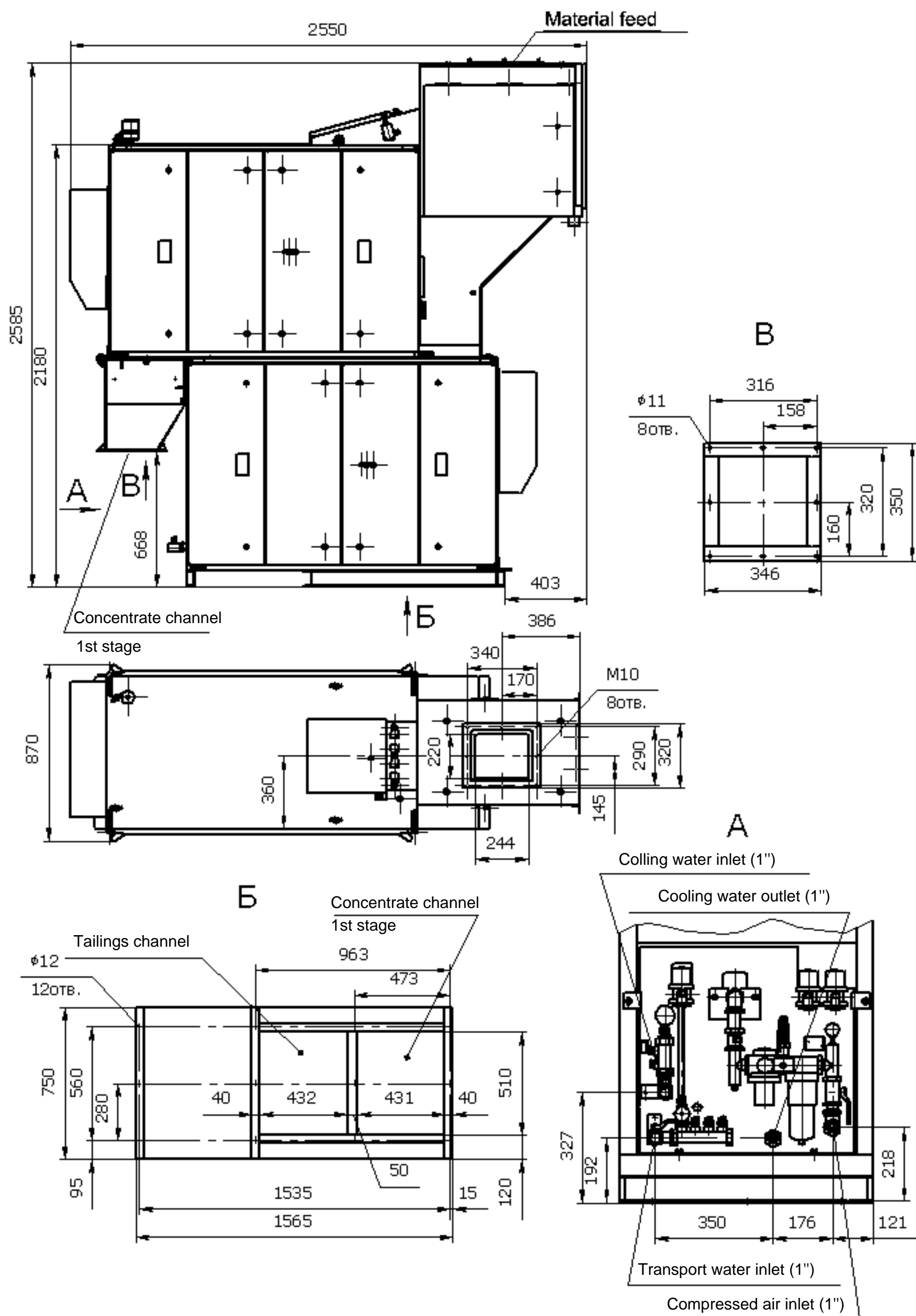
Sorting machine LS-50-05
